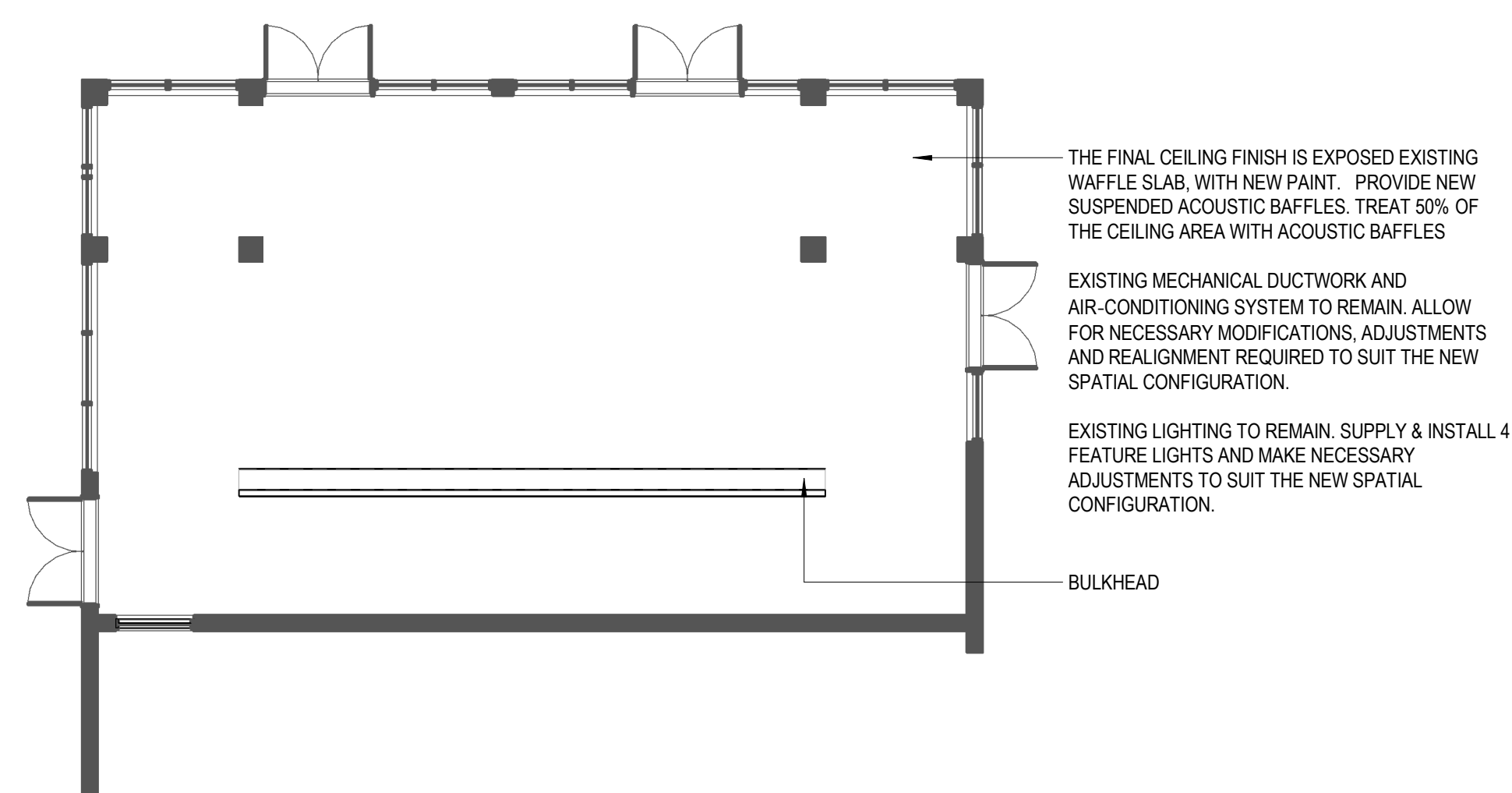
2 31-00 GROUND FLOOR - CEILING PLAN - GROUND FLOOR 1 : 100
